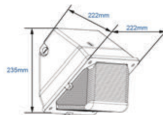
LED Pro Large Civic Optics: IES Type IV
